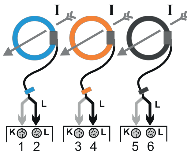
Fig. 2 Connection with EM210
